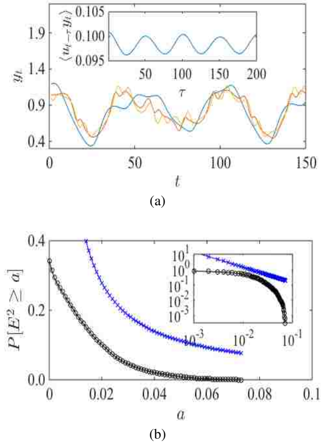
Figure 3.4: Target output and system output generated with analytical weights and trained weights for the Mackey-Glass 10 step ahead prediction task (a), the worst-case bounds using the Markov inequality, with the same plot on a log-log scale in the inset (b).
